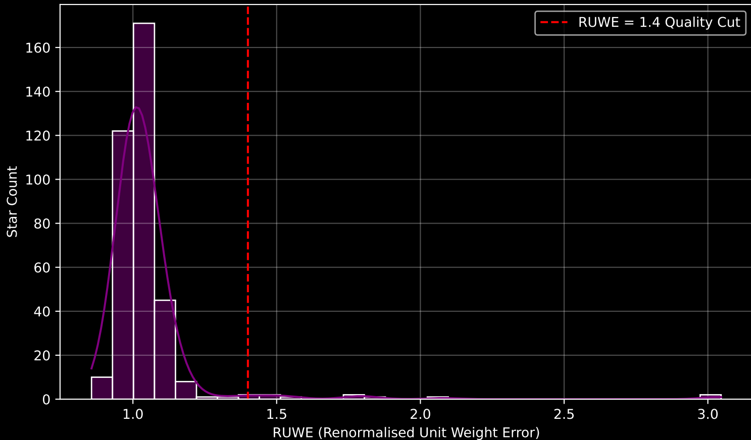
GAPOGEE DR17 Field [266-06] RUWE Distribution (n= 369)
