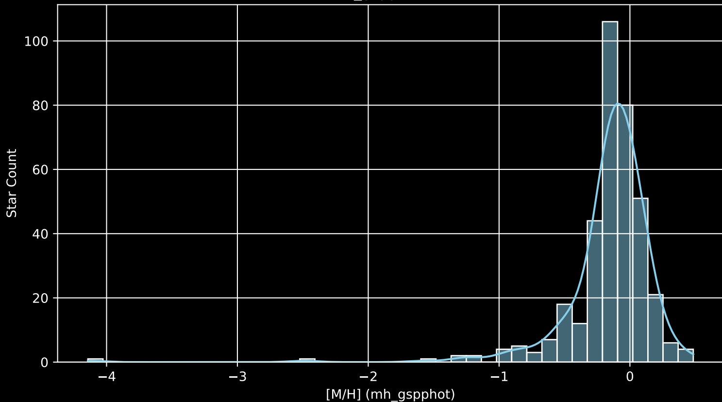
APOGEE DR17 Field: [266-06 [M/H] (mh_gspphot) (n= 368)
