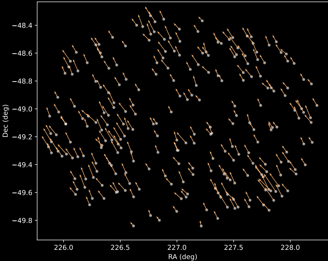
APOGEE DR17 Cluster 3 Proper Motion Vectors (n=249)
