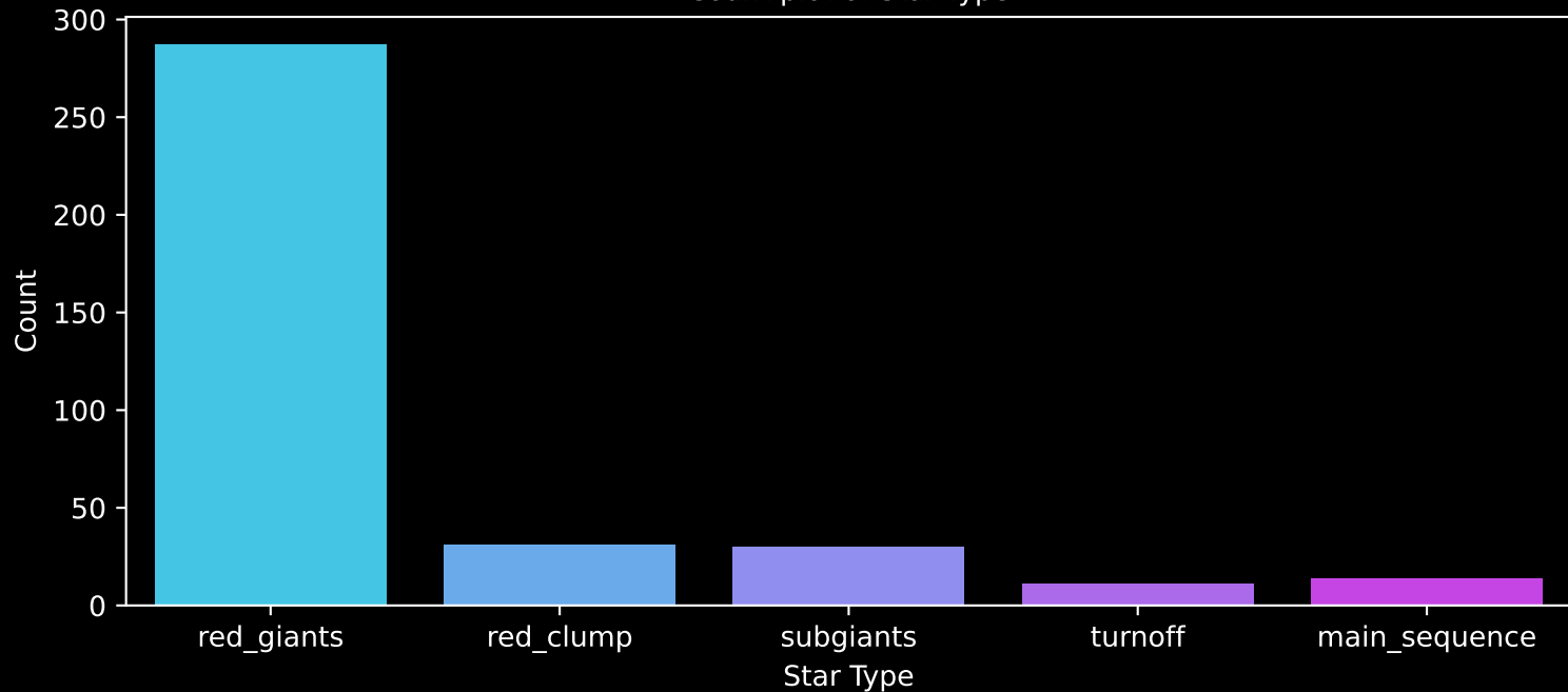
APOGEE DR17 Field: [266-06] Count plot of Star Type
