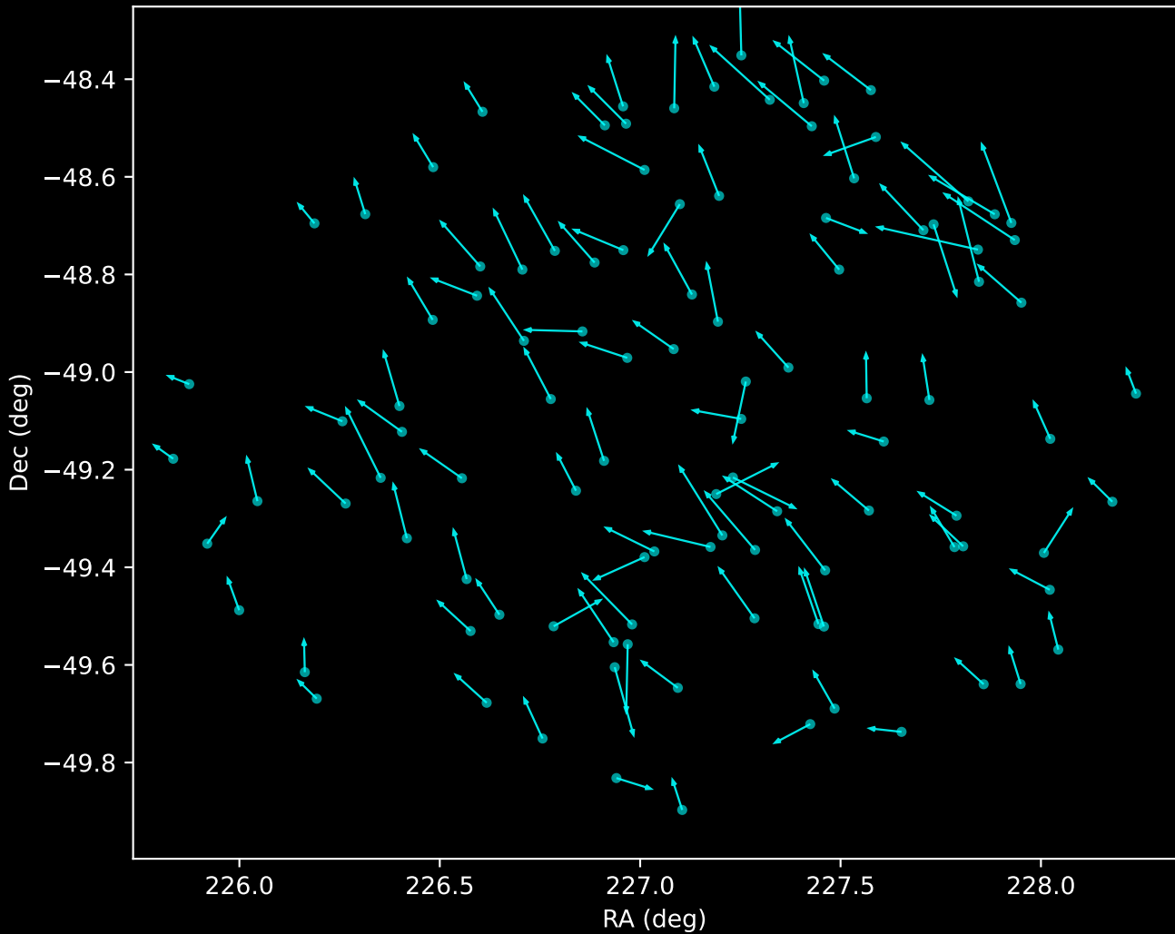
APOGEE DR17 Noise Stream Proper Motion Vectors (n=107)
