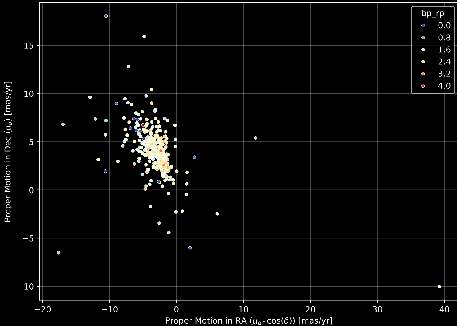
APOGEE DR17 Field: [266-06] Proper Motion Diagram (n= 373)
