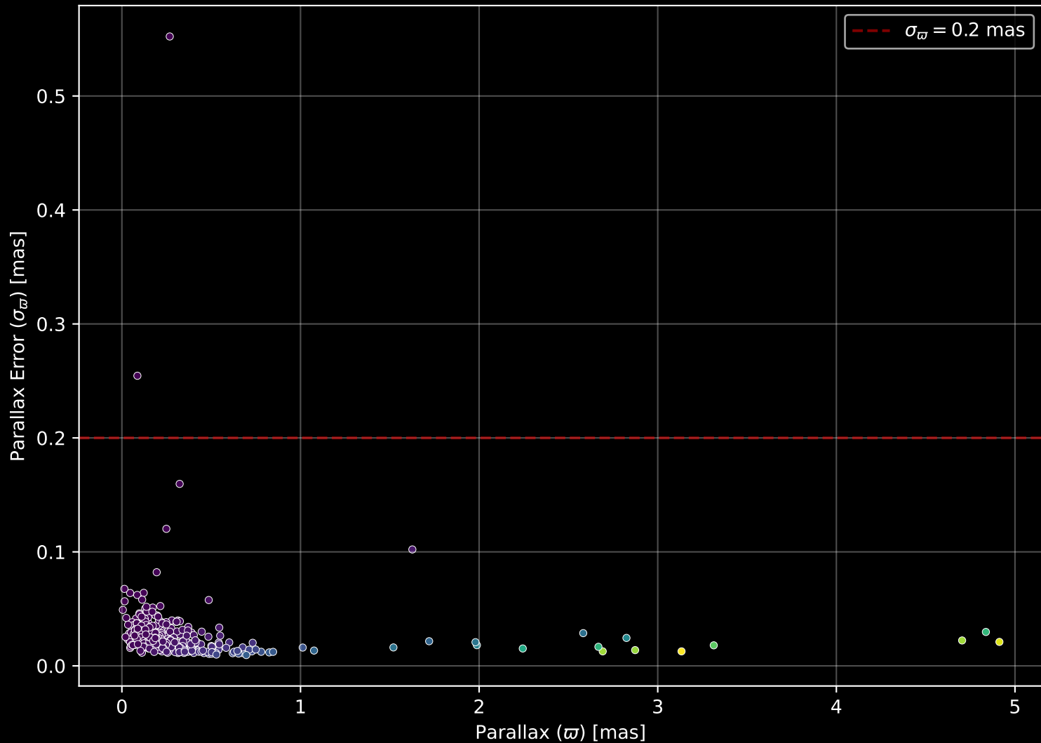
APOGEE DR17 Field: [266-06] Parallax Quality (n= 373)
